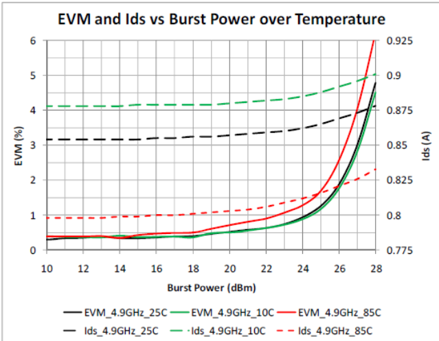
Figure 9 EVM vs Burst Power and Temperature
