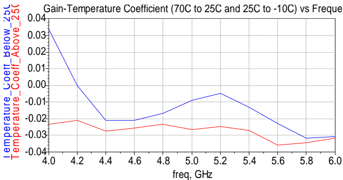
Figure 7 Gain-Temperature Coefficient
