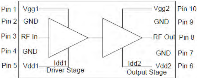
Figure 1 Functional Diagram
