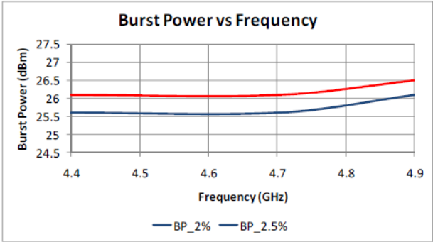
Figure 5 Burst Power
